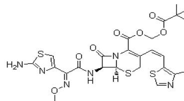
Chemical Structure
