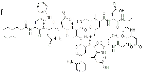
Chemical Structure
