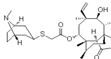
Chemical Structure
