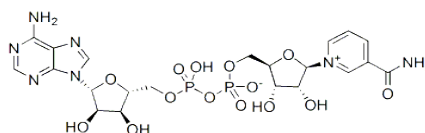
Chemical Structure
