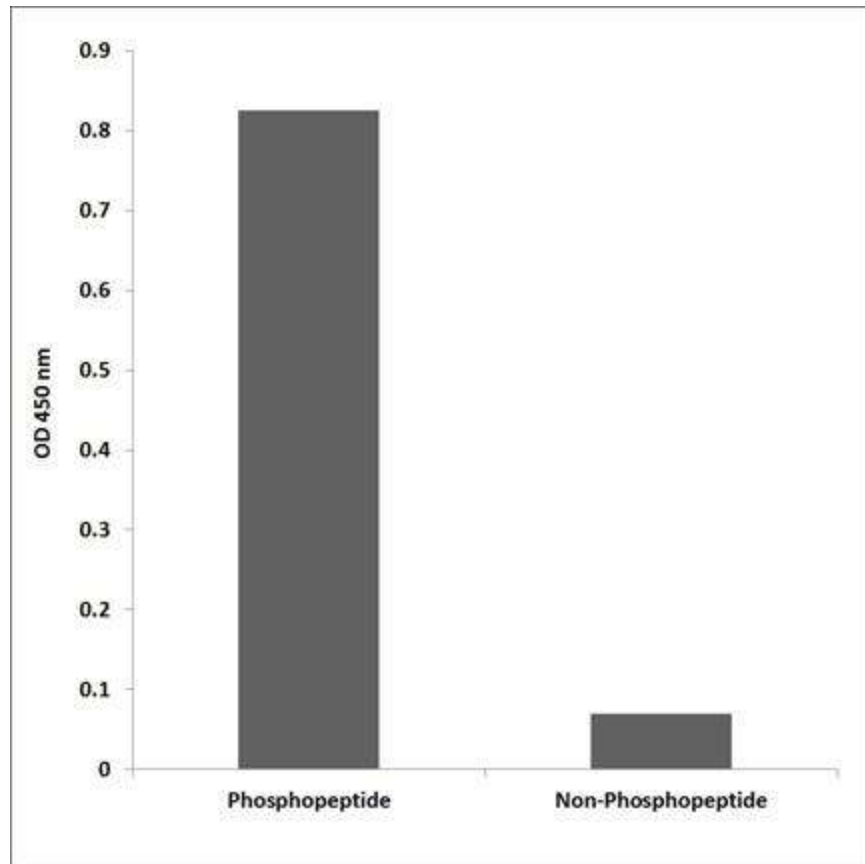
Figure 3. Enzyme-Linked Immunosorbent Assay (ELISA) for immunogen phosphor-peptide (left) and non-phosphopeptide (right), using Anti-ALK (Phospho-Tyr1507) Antibody.
