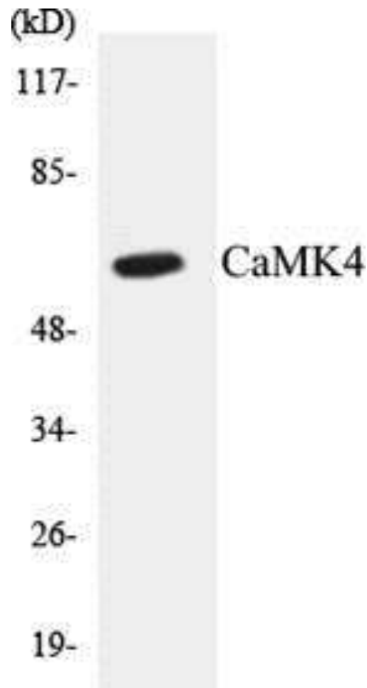
Figure 4. Western blot analysis of extracts from K562 cells, treated with H 2 O 2 100uM 30', using the Anti-CaMK4 Antibody.
