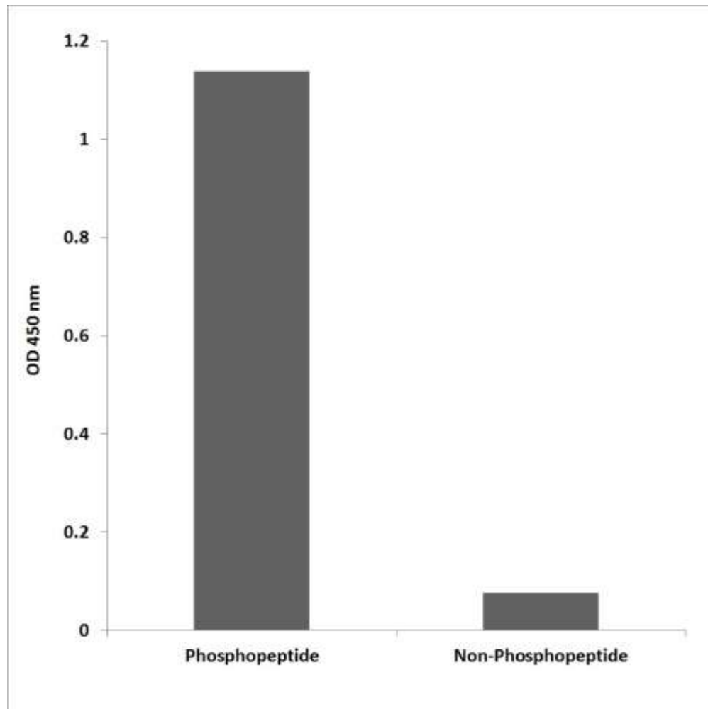
Figure 3. Enzyme-Linked Immunosorbent Assay (ELISA) for immunogen phosphor-peptide (left) and non-phospho peptide (right), using Anti-CaMK4 (Phospho-Thr196/200) Antibody.
