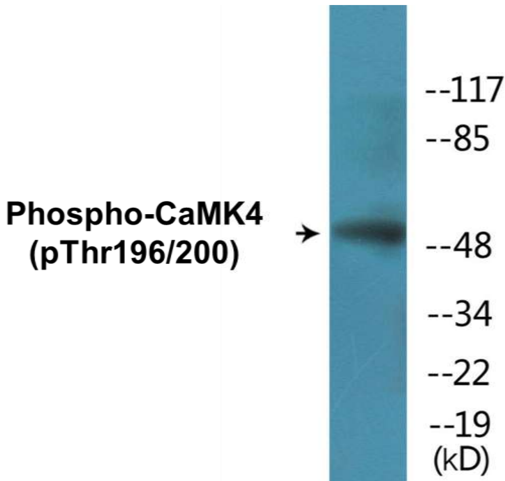
Figure 2. Western blot analysis of extracts from K562 cells treated with H 2 O 2 100uM 30', using the Anti-CaMK4 (Phospho-Thr196/200) Antibody.
