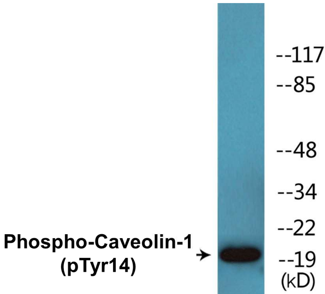
Figure 2. Western blot analysis of extracts from HuvEc cells treated with PMA 125ng/ml 30' and HeLa cells treated with LPS 100ng/ml 30', using the Anti-Caveolin-1 (Phospho-Tyr14) Antibody.
