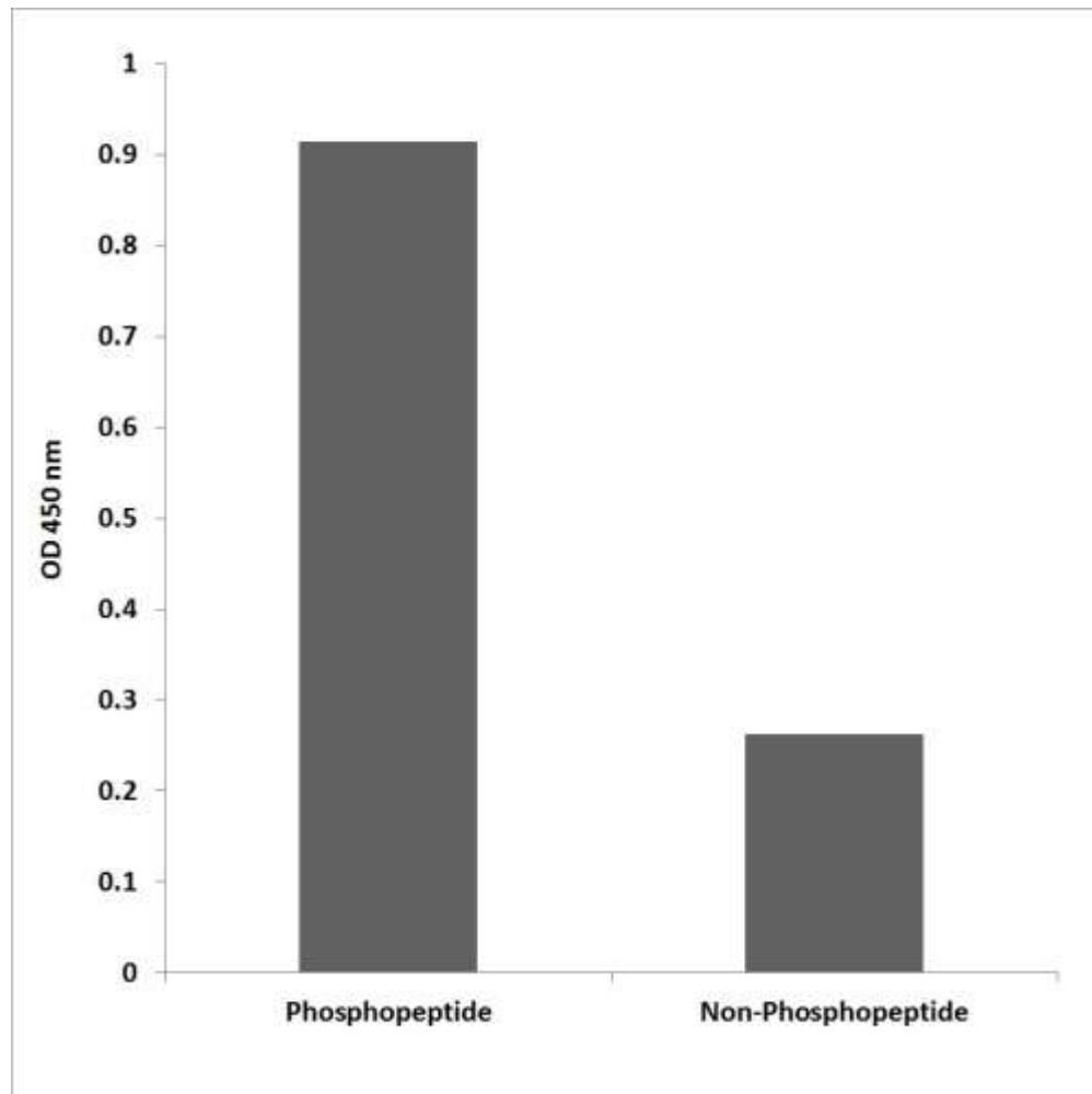
Figure 3. Enzyme-Linked Immunosorbent Assay (ELISA) for immunogen phosphor-peptide (left) and non-phospho peptide (right), using Anti-Caveolin-1 (Phospho-Tyr14) Antibody.
