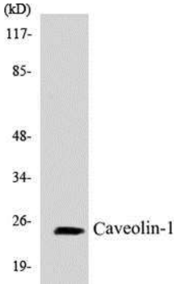
Figure 4. Western blot analysis of extracts from NIH-3T3 cells, using the Anti-Caveolin-1 Antibody.
