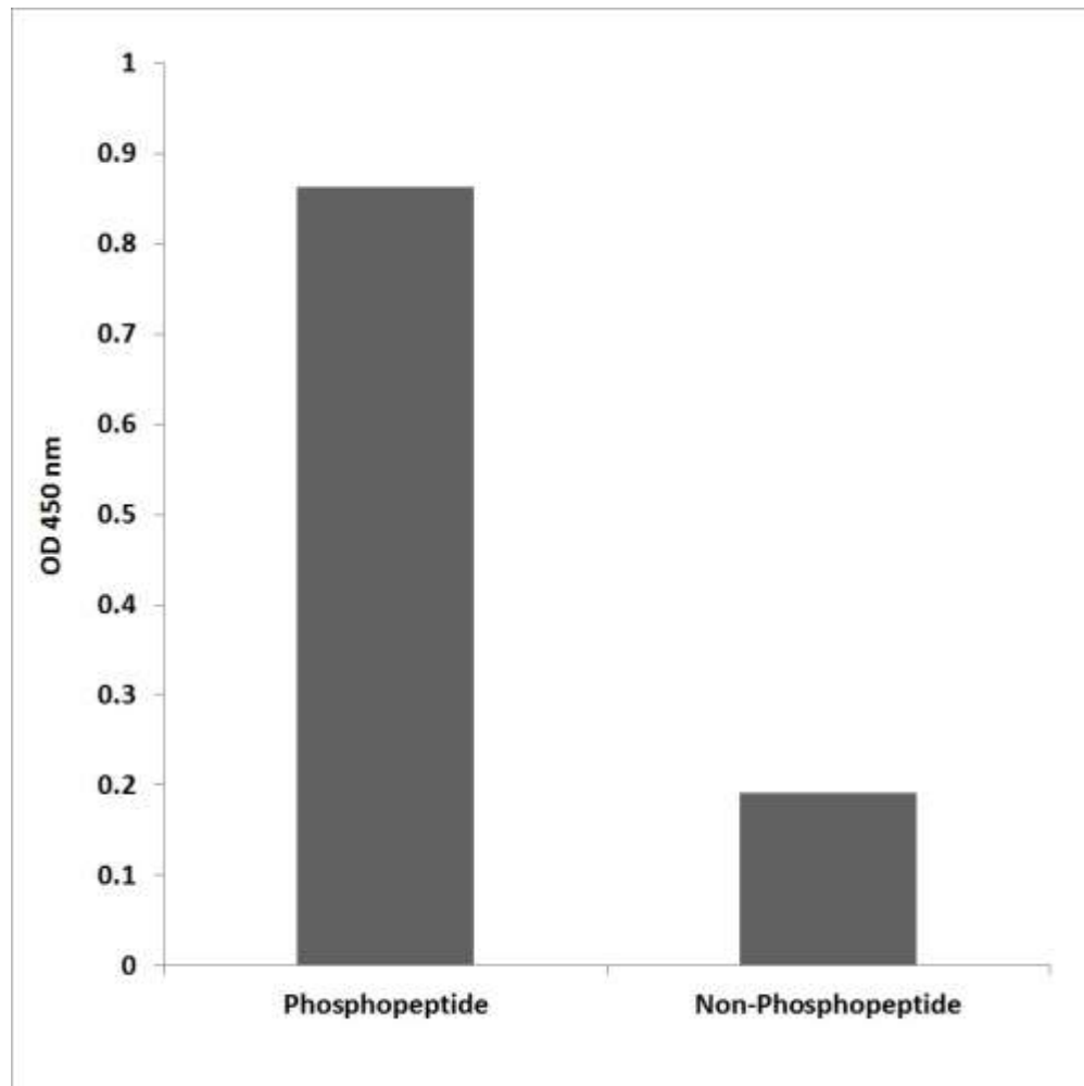
Figure 3. Enzyme-Linked Immunosorbent Assay (ELISA) for immunogen phosphor-peptide (left) and non-phospho peptide (right), using Anti-p53 (Phospho-Ser378) Antibody.
