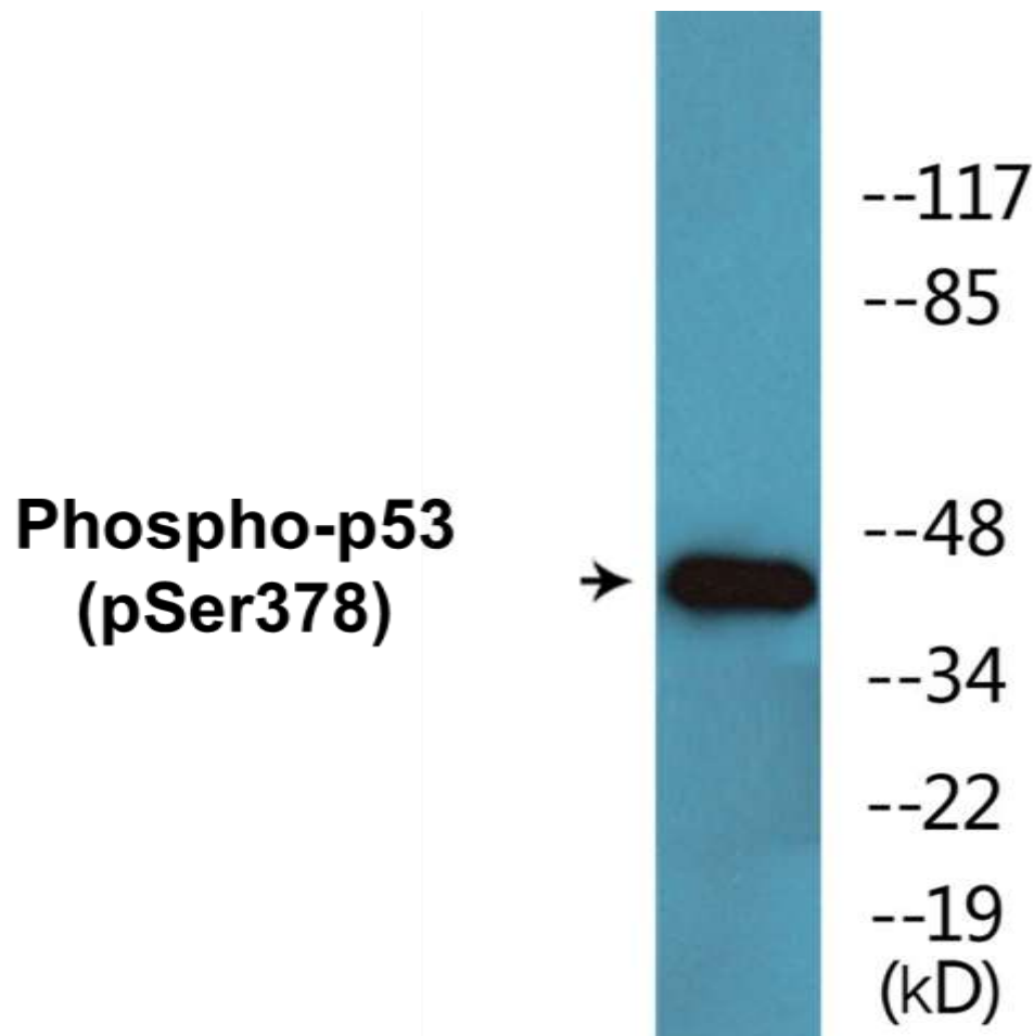
Figure 2. Western blot analysis of extracts from Jurkat cells treated with UV 15', using the Anti-p53 (Phospho-Ser378) Antibody.
