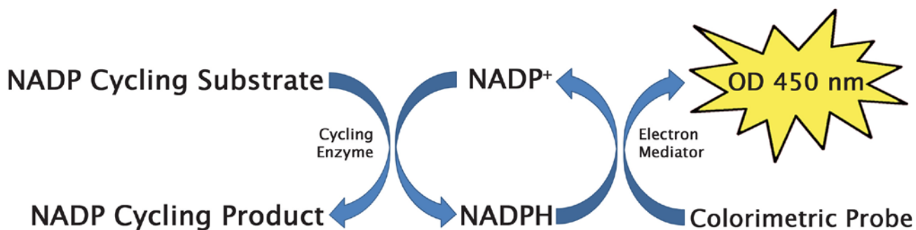
Figure 1. NADP + /NADPH Cycling Assay Principle.
