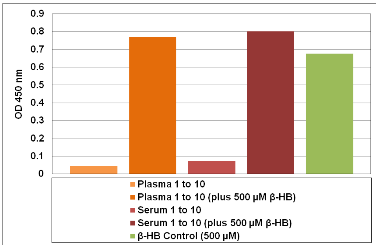
Figure 3: β-Hydroxybutyrate Detection. Normal human plasma and serum were both diluted 1:10 in 1X Assay Buffer and tested with and without 500 µM β-Hydroxybutyrate spiked into them. The samples were tested according to the assay protocol. Background values have been subtracted.
