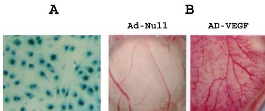
Figure 2: A. X-gal staining of infected HUVEC cells. HUVEC cells were infected with purified Ad- \beta Gal at 50 MOI (multiplicity of infection). X-gal staining was performed after 48 hr infection period. B. VEGF-induced Angiogenesis. Purified Ad-Null or Ad-VEGF viruses were applied to a 10-day old CAM (chick chorioallantoic membrane). After three days, the blood vessels on the CAM were examined under a stereomicroscope.
