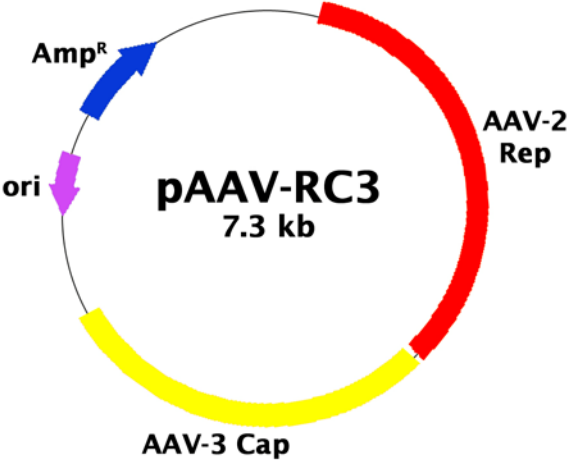
Figure 3. pAAV-RC3 Vector
