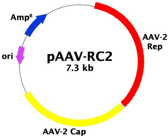
Figure 5. pAAV-RC2 Vector
