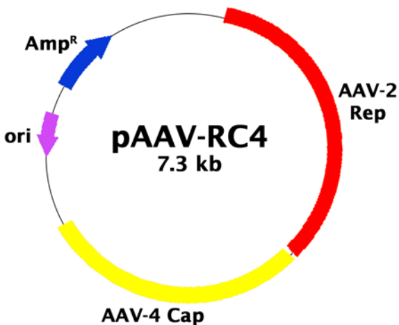
Figure 5. pAAV-RC4 Vector
