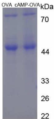
Figure 1. SDS-PAGE
