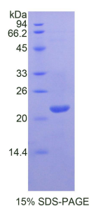
Figure. SDS-PAGE
