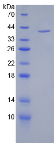
Figure 1. SDS-PAGE
