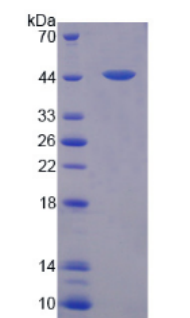
Figure. SDS-PAGE
