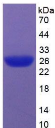
Figure 1. SDS-PAGE
