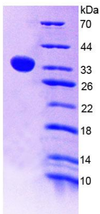
Figure 1. SDS-PAGE
