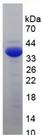
Figure 2. SDS-PAGE
