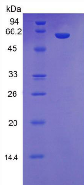
Figure 2. SDS-PAGE
