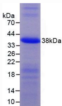
Figure 1. SDS-PAGE
