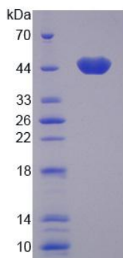
Figure 1. SDS-PAGE
