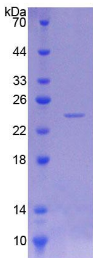
Figure 1. SDS-PAGE
