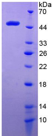
Figure 2. SDS-PAGE
