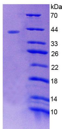
Figure 1. SDS-PAGE
