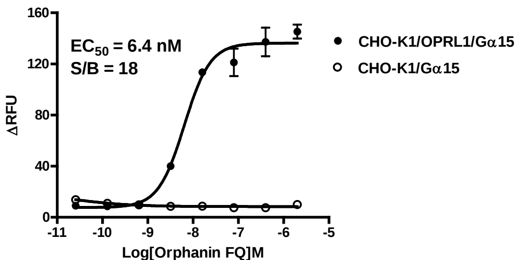
Figure 1. Orphanin FQ-induced concentration-dependent stimulation of intracellular calcium mobilization in CHO-K1/OPRL1/Gα15 and CHO-K1/Gα15 cells. The cells were loaded with Calcium-4 prior to stimulation with an OPRL1 receptor agonist, Orphanin FQ. The intracellular calcium change was measured by FlexStation. The relative fluorescent units (RFU) were plotted against the log of the cumulative doses (5-fold dilution) of Orphanin FQ (Mean ± SD, n = 2). The EC 50 of Orphanin FQ on OPRL1 co-expressing with Gα15 in CHO-K1 cells was 6.4 nM. The S/B of Orphanin FQ on OPRL1 co-expressing with Gα15 in CHO-K1 cells was 18.
