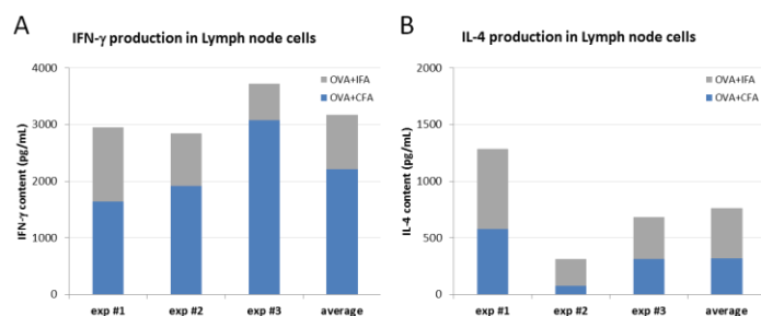
Figure 2. CFA adjuvant favors a strong Th1 response. BALB/c mice were immunized with OVA+IFA or OVA+CFA and draining lymph nodes were harvested 7 days later. (A) IFN-γ and (B) IL-4 production was measured by ELISA after 72H in vitro incubation with OVA (adapted from Shibaki et al. Exp Derm. 2002;11:163-134).
