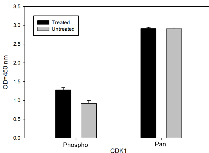
Fig. 3 HELA cells were stimulated by Hydroxyurea for 24 hours at 37°C
