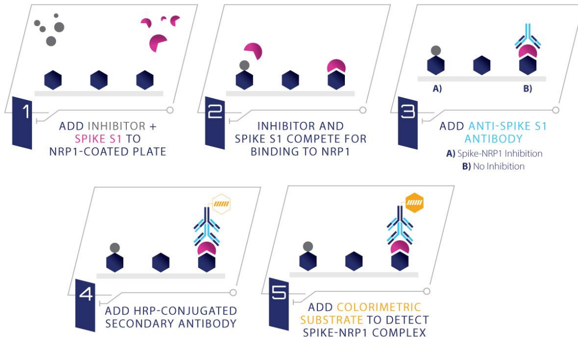
A schematic showing how the RayBio® Spike-NRP1 Binding Assay Kit can measure the inhibition of the Spike S1 subunit and NRP1 in the presence of a potential inhibitor.
