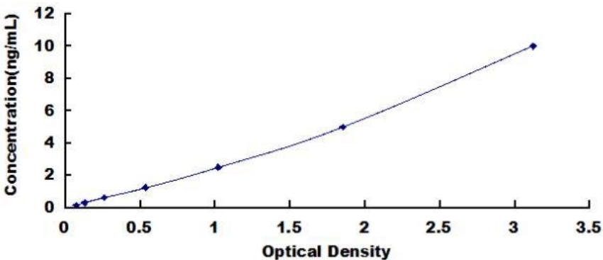
Typical Standard Curve for Human COL1a2 ELISA.
