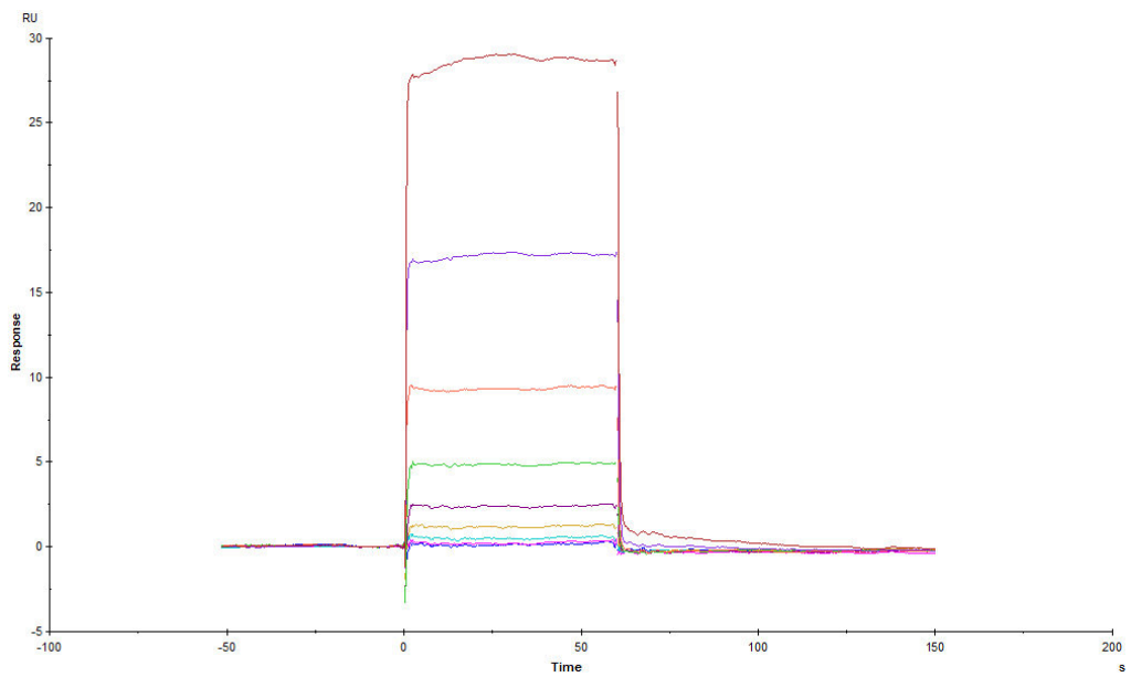
Mink ACE2, His Tag (Cat. No. AC2-M52H3) immobilized on CM5 Chip can bind SARS-CoV-2 S protein RBD, His Tag (Cat. No. SPD-C52H3) with an affinity constant of 8.34 \mu M as determined in a SPR assay (Biacore T200) (Routinely tested).
