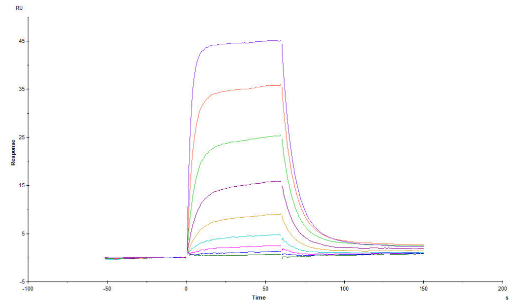
Mink ACE2, His Tag (Cat. No. AC2-M52H3) immobilized on CM5 Chip can bind SARS-CoV-2 S protein RBD (Y453F), His Tag with an affinity constant of 0.178 \mu M as determined in a SPR assay (Biacore T200) (QC tested).
