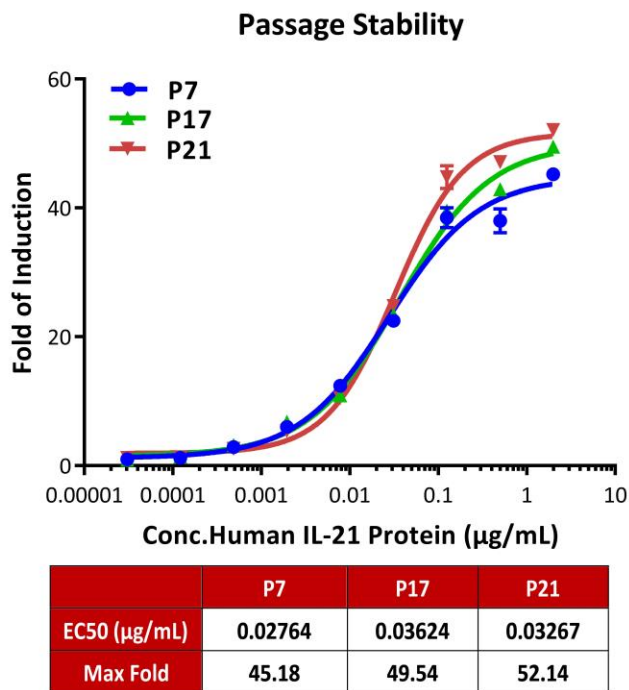
Fig5. Passage stability analysis by Signaling Bioassay. The continuously growing Human IL-21 R/CD132 (Luc) HEK293 Reporter Cell was stimulated with serial dilutions of human IL-21 protein (Cat. No. IL1-H5213). Human IL-21 protein stimulated response demonstrates passage stabilization (fold induction and EC50) across passage 7-21.
