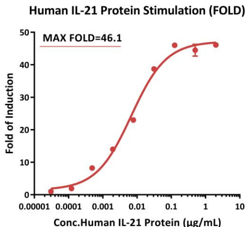
Fig3. Response to human IL-21 protein (FOLD). The Human IL-21 R /CD132 (Luc) HEK293 Reporter Cell was stimulated with serial dilutions of human IL-21 protein (Cat. No. IL1-H5213). The max induction fold was approximately 46.1.
