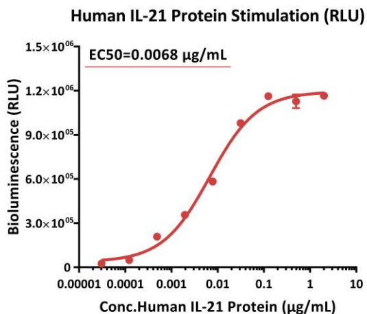
Fig2. Response to human IL-21 protein (RLU). The Human IL-21 R/CD132 (Luc) HEK293 Reporter Cell was stimulated with serial dilutions of human IL-21 protein (Cat. No. IL1-H5213). The EC 50 was approximately 0.0068 µg/mL.
