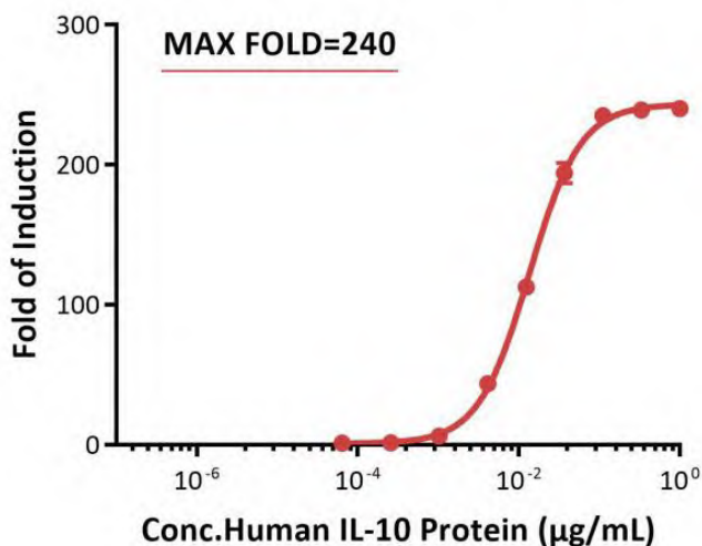
Fig3. Response to human IL-10 protein (FOLD). The Human IL-10 R alpha/IL-10 R beta (Luc) HEK293 Reporter Cell was stimulated with serial dilutions of human IL-10 protein (Cat. No. IL0-H5219). The max induction fold was approximately 240.
