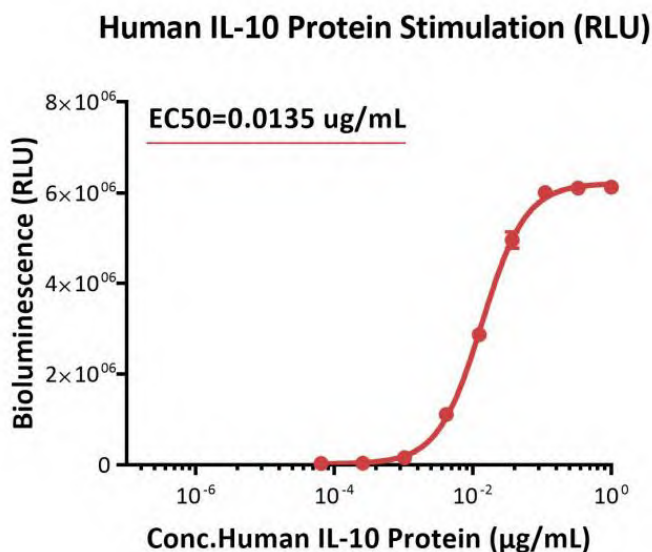
Fig2. Response to human IL-10 protein (RLU). The Human IL-10 R alpha/IL-10 R beta (Luc) HEK293 Reporter Cell was stimulated with serial dilutions of human IL-10 protein (Cat. No. IL0-H5219). The EC 50 was approximately 0.0135 µg/mL.
