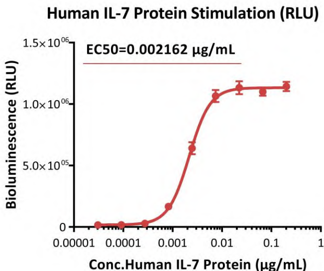
Fig2. Response to human IL-7 protein (RLU). The Human IL-7 R alpha/CD132 (Luc) HEK293 Reporter Cell was stimulated with serial dilutions of human IL-7 protein (Cat. No. IL7-H4219). The EC 50 was approximately 0.002162 µg/mL.
