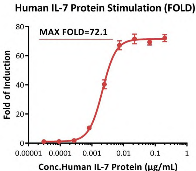
Fig3. Response to human IL-7 protein (FOLD). The Human IL-7 R alpha/CD132 (Luc) HEK293 Reporter Cell was stimulated with serial dilutions of human IL-7 protein (Cat. No. IL7-H4219). The max induction fold was approximately 72.1.
