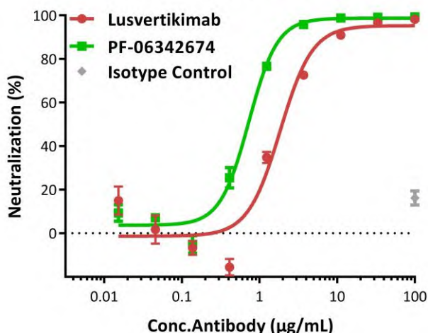
Fig4. Inhibition of human IL-7 protein-induced reporter activity by anti-human IL-7 R neutralizing antibody. This reporter cell was incubated with serial dilutions of antibodies in the presence of human IL-7 protein (Cat. No. IL7-H4219) with a final concentration of 0.002 µg/mL. The EC50 of Lusvertikimab is approximately 1.844 µg/mL, and the EC50 of PF-06342674 is approximately 0.729 µg/mL.
