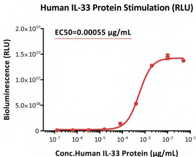
Fig2. Response to human IL-33 protein (RLU). The Human IL-1 R1 & IL-1 RAcP (IL-33 receptor) (Luc) HEK293 Reporter Cell was stimulated with serial dilutions of human IL-33 protein (Cat. No. IL3-H52H7). The EC 50 was approximately 0.00055 µg/mL.
