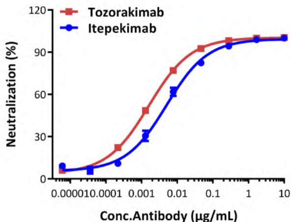
Fig4. Inhibition of human IL-33 protein-induced reporter activity by anti-human IL-33 neutralizing antibody. This reporter cell was incubated with serial dilutions of anti-human IL-33 neutralizing antibodies in the presence of human IL-33 protein (Cat. No. IL3-H52H7) with a final concentration of 0.0001 µg/mL. The EC50 of Tozorakimab is approximately 0.0016 µg/mL, and the EC50 of Itepekimab is approximately 0.0050 µg/mL.
