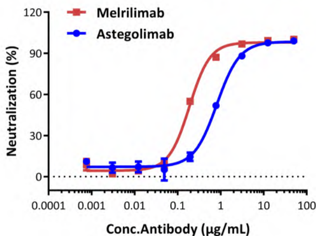
Fig5. Inhibition of human IL-33 protein-induced reporter activity by anti-human IL-1RL1 neutralizing antibody. This reporter cell was incubated with serial dilutions of anti-human IL-1RL1 neutralizing antibodies in the presence of human IL-33 protein (Cat. No. IL3-H52H7) with a final concentration of 0.0001 µg/mL. The EC50 of Melrilimab is approximately 0.1882 µg/mL, and the EC50 of Astegolimab is approximately 0.8173 µg/mL.
