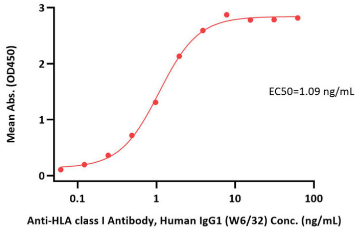
Biotinylated Human HLA-B*07:02&B2M&HPV16 E7 (KPTLKEYVL) Complex Protein ELISA 0.1 µg of Biotinylated Human HLA-B*07:02&B2M&HPV16 E7 (KPTLKEYVL) Complex Protein per well
