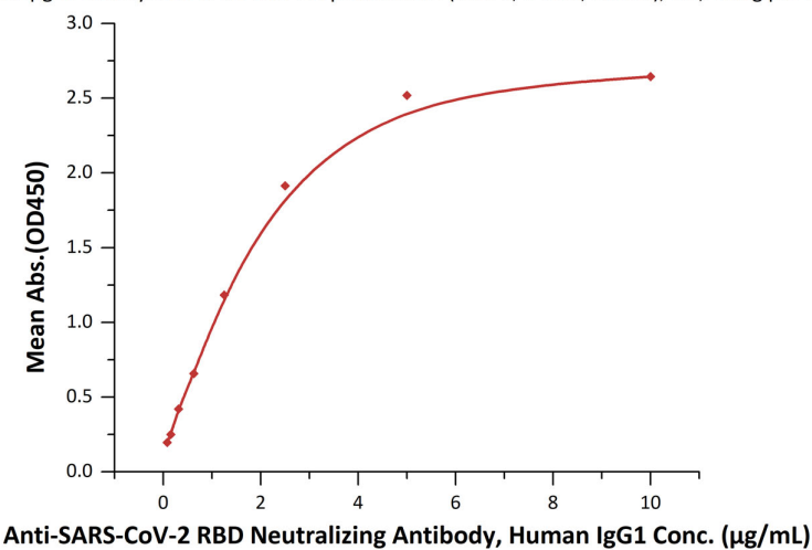
Biotinylated SARS-CoV-2 S protein RBD (K417T, E484K, N501Y), His,Avitag ELISA 0.1 µg of Biotinylated SARS-CoV-2 S protein RBD (K417T, E484K, N501Y), His,Avitag per well
