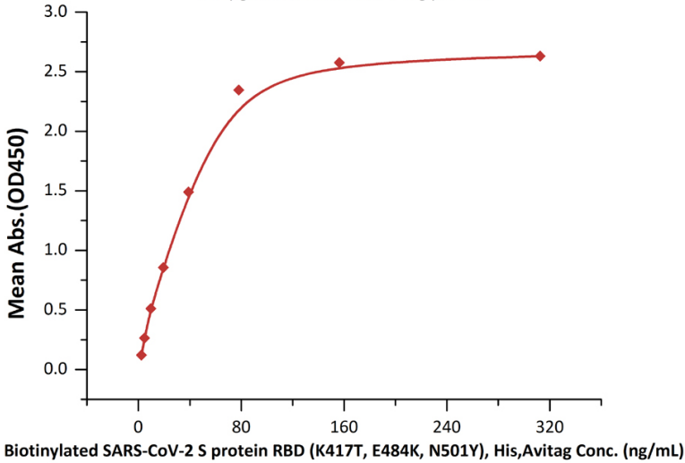
Biotinylated SARS-CoV-2 S protein RBD (K417T, E484K, N501Y), His,Avitag ELISA 0.1 µg of Human ACE2, Fc Tag per well
