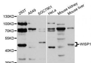
Western blot analysis of extracts of various cell lines, using WISP1 antibody (abx002388) at 1/1000 dilution.
