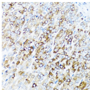
Immunohistochemistry of paraffin-embedded mouse stomach using SERPINA7 antibody (abx006337) at dilution of 1/100 (40x lens).
