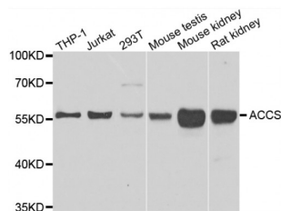
Western blot analysis of extracts of various cell lines, using ACCS antibody (abx006477) at 1/1000 dilution.
