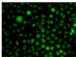
Immunofluorescence analysis of A549 cells using UBE2R2 antibody (abx006931).
