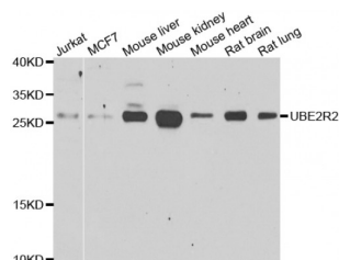
Western blot analysis of extracts of various cell lines, using UBE2R2 antibody (abx006931) at 1/1000 dilution.
