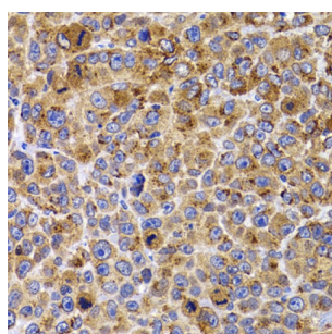
Immunohistochemistry of paraffin-embedded mouse cancer using UBE2R2 antibody (abx006931) at dilution of 1/100 (40x lens).
