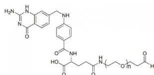
Chemical structure of FA-PEG-CHO.
