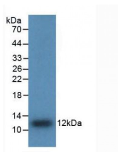
Western blot analysis of recombinant Human IL8.
