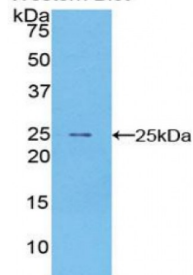
Western Blot
