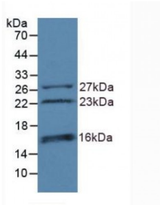
Western blot analysis of recombinant Human CHD3.
