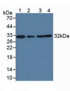
Western blot analysis of (1) Cow Heart Tissue, (2) Cow Liver Tissue, (3) Human HeLa cells and (4) Human K-562 Cells.
