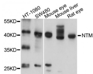
Western blot analysis of extracts of various cell lines, using NTM antibody (abx123694) at 1/1000 dilution.
