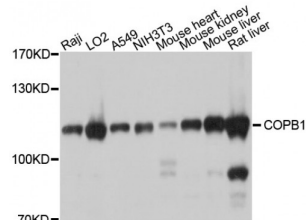
Western blot analysis of extracts of various cell lines, using COPB1 antibody (abx125701) at 1/1000 dilution.
